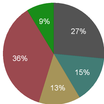
Tennessee Energy Consumption, 2010 Consumption by Fuel Type (%)
