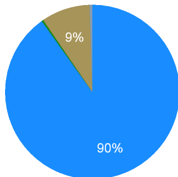
Tennessee Renewable Electricity Generation, 2011
