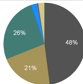
Georgia Electricity Generation, 2011
