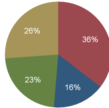
Arkansas Energy Consumption, 2010 Consumption by Sector (%)
