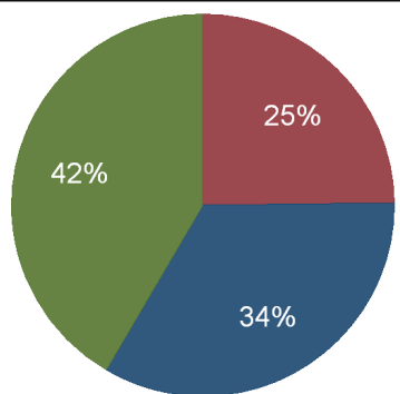
SSEB Region Electricity Consumption, 2011 Consumption by Sector (%)
