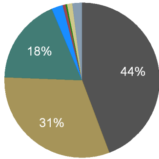
SSEB Region Electricity Generation, 2011 Electricity Generation by Fuel Type (%)
