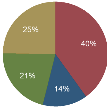
Alabama Energy Consumption, 2010 Consumption by Sector (%)
