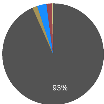
Kentucky Electricity Generation, 2011
