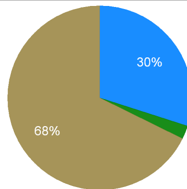
Louisiana Renewable Electricity Generation, 2011
