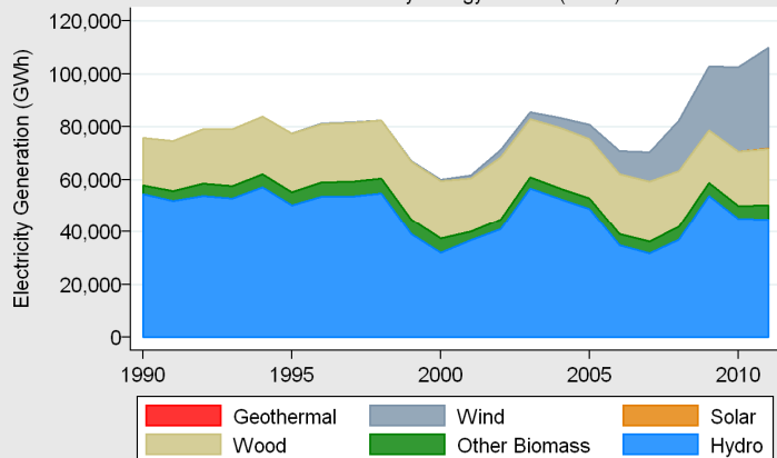
SSEB Region Renewable Electricity Generation, 1990-2011 Generation by Energy Source (GWh)
