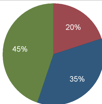
North Carolina Electricity Consumption, 2011 Consumption by Sector (%)
