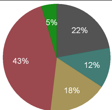
Maryland Energy Consumption, 2010
