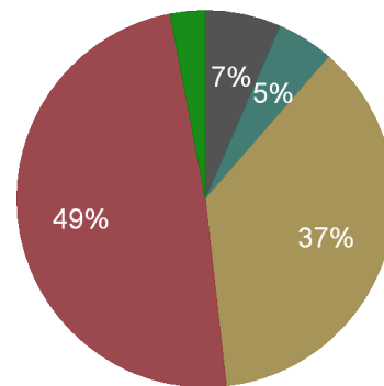
Louisiana Energy Consumption, 2010 Consumption by Fuel Type (%)
