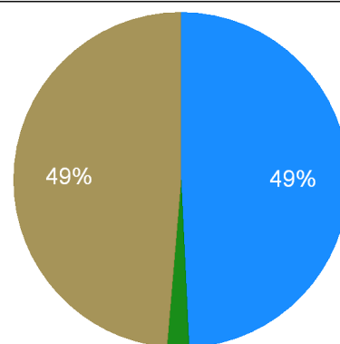
Georgia Renewable Electricity Generation, 2011
