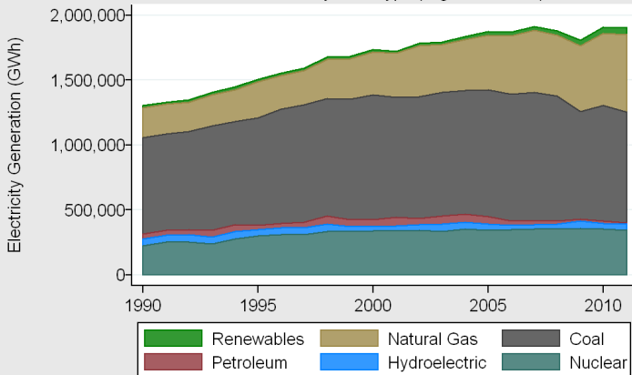
SSEB Region Electricity Generation, 1990-2011 Generation by Fuel Type (Gigawatt Hours)
