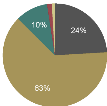
Florida Electricity Generation, 2011
