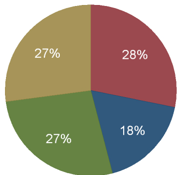
Tennessee Energy Consumption, 2010 Consumption by Sector (%)
