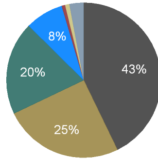
United States Electricity Generation, 2011 Electricity Generation by Fuel Type (%)
