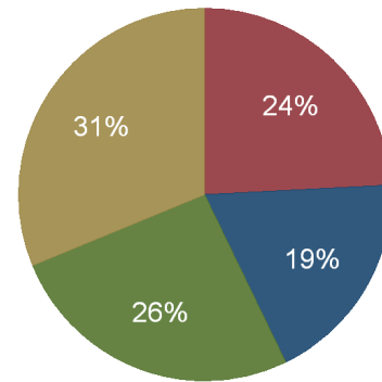
Georgia Energy Consumption, 2010 Consumption by Sector (%)
