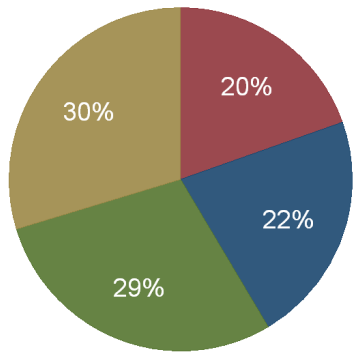
Missouri Energy Consumption, 2010 Consumption by Sector (%)
