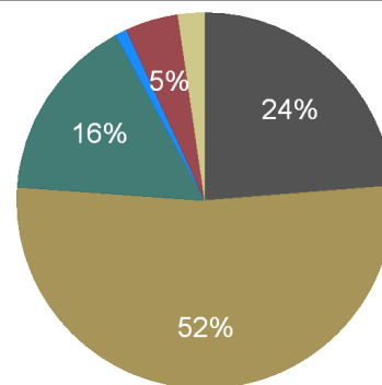
Louisiana Electricity Generation, 2011
