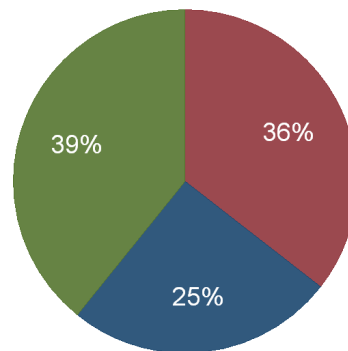
Arkansas Electricity Consumption, 2011 Consumption by Sector (%)
