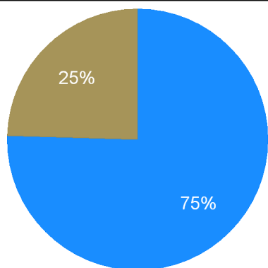
Alabama Renewable Electricity Generation, 2011
