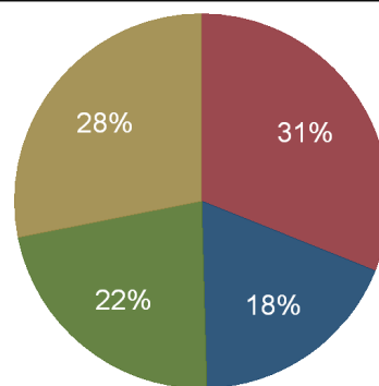
United States Energy Consumption, 2010 Consumption by Sector (%)
