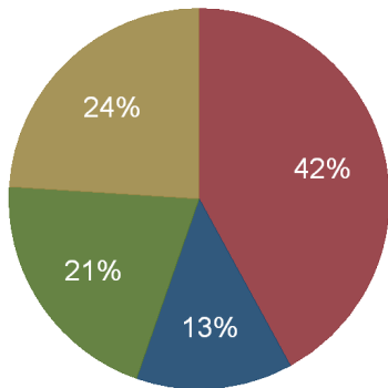
Kentucky Energy Consumption, 2010 Consumption by Sector (%)
