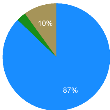
Kentucky Renewable Electricity Generation, 2011
