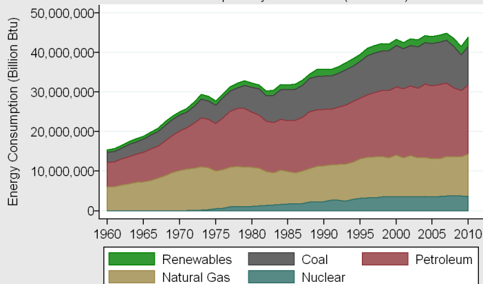
SSEB Region Energy Consumption, 1960-2010 Consumption by Fuel Source (Billion Btu)
