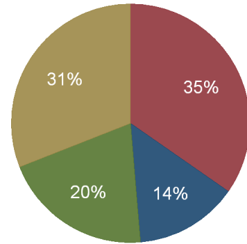
Mississippi Energy Consumption, 2010 Consumption by Sector (%)
