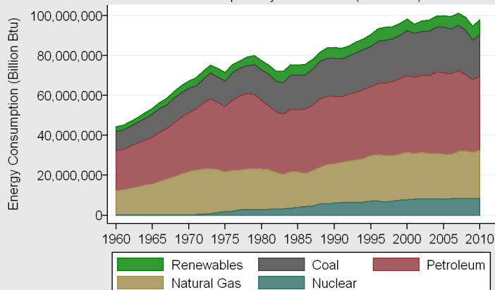
United States Energy Consumption, 1960-2010 Consumption by Fuel Source (Billion Btu)
