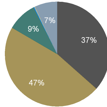
Texas Electricity Generation, 2011 Electricity Generation by Fuel Type (%)
