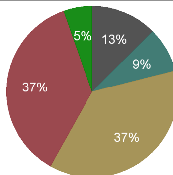
Mississippi Energy Consumption, 2010
