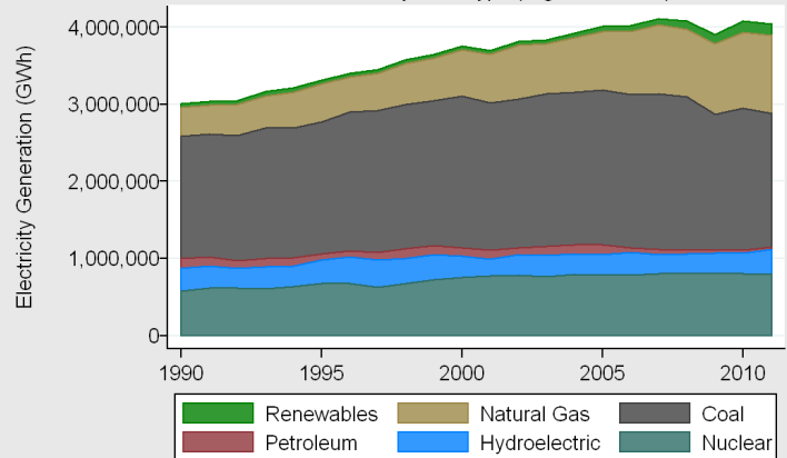
United States Electricity Generation, 1990-2011 Generation by Fuel Type (Gigawatt Hours)
