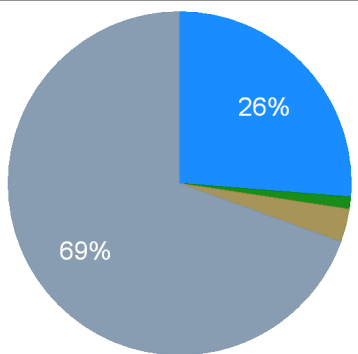
Oklahoma Renewable Electricity Generation, 2011
