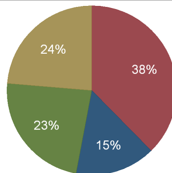
West Virginia Energy Consumption, 2010 Consumption by Sector (%)
