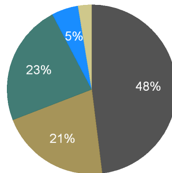
Arkansas Electricity Generation, 2011
