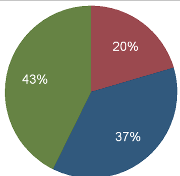
Missouri Electricity Consumption, 2011 Consumption by Sector (%)
