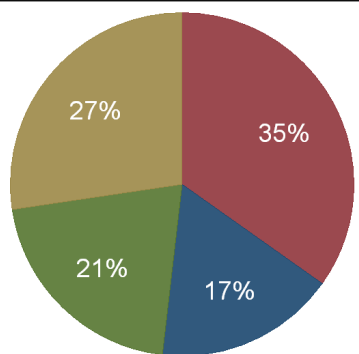
SSEB Region Energy Consumption, 2010 Consumption by Sector (%)
