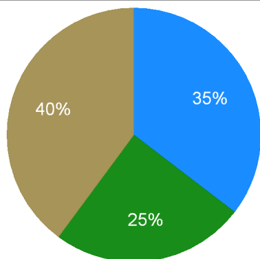
Virginia Renewable Electricity Generation, 2011
