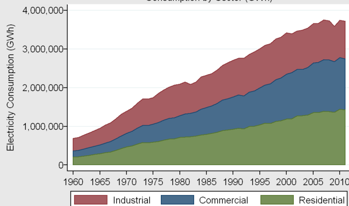
United States Electricity Consumption, 1960-2011 Consumption by Sector (GWh)
