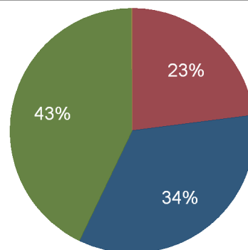
Georgia Electricity Consumption, 2011 Consumption by Sector (%)
