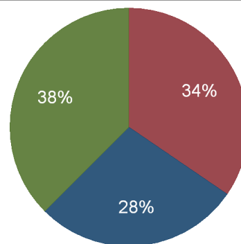
Louisiana Electricity Consumption, 2011 Consumption by Sector (%)
