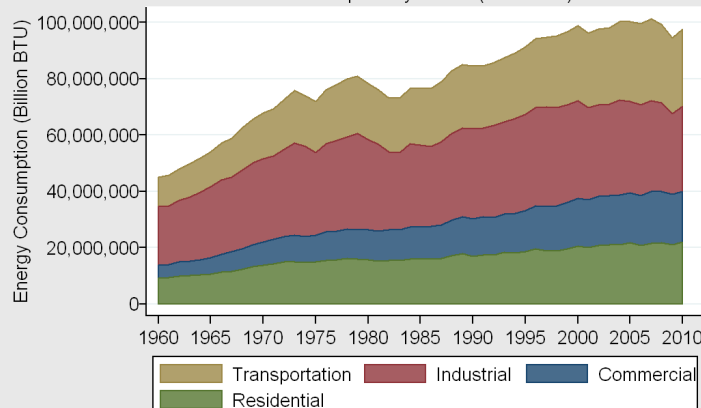
United States Energy Consumption, 1960-2010 Consumption by Sector (Billion Btu)
