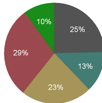
Arkansas Energy Consumption, 2010 Consumption by Fuel Type (%)
