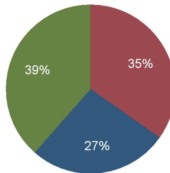
South Carolina Electricity Consumption, 2011 Consumption by Sector (%)
