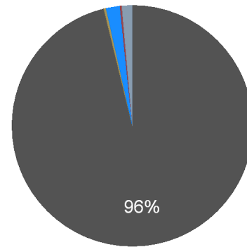
West Virginia Electricity Generation, 2011 Electricity Generation by Fuel Type (%)
