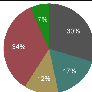
North Carolina Energy Consumption, 2010
