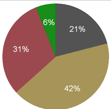
Oklahoma Energy Consumption, 2010
