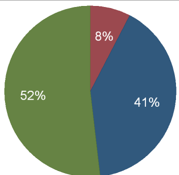
Florida Electricity Consumption, 2011 Consumption by Sector (%)
