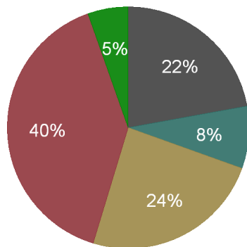
SSEB Region Energy Consumption, 2010 Consumption by Fuel Type (%)
