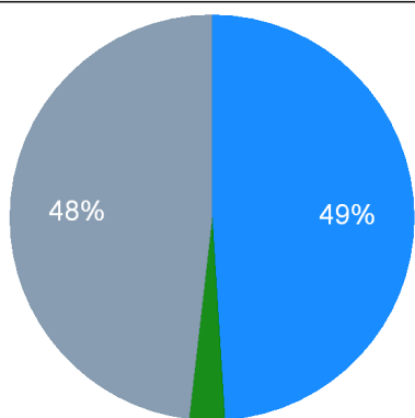
Missouri Renewable Electricity Generation, 2011
