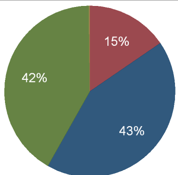
Virginia Electricity Consumption, 2011 Consumption by Sector (%)
